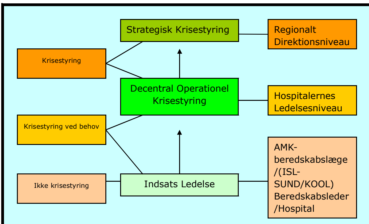
Figur 2: Krisestyring
